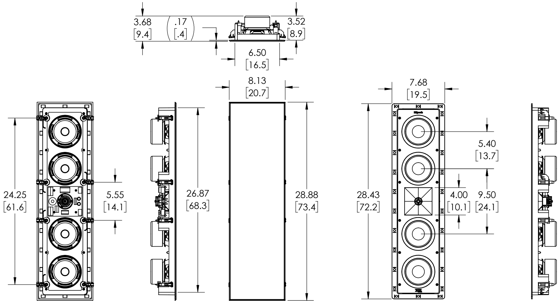
UNCLAMPED SHIPPING POSITION
